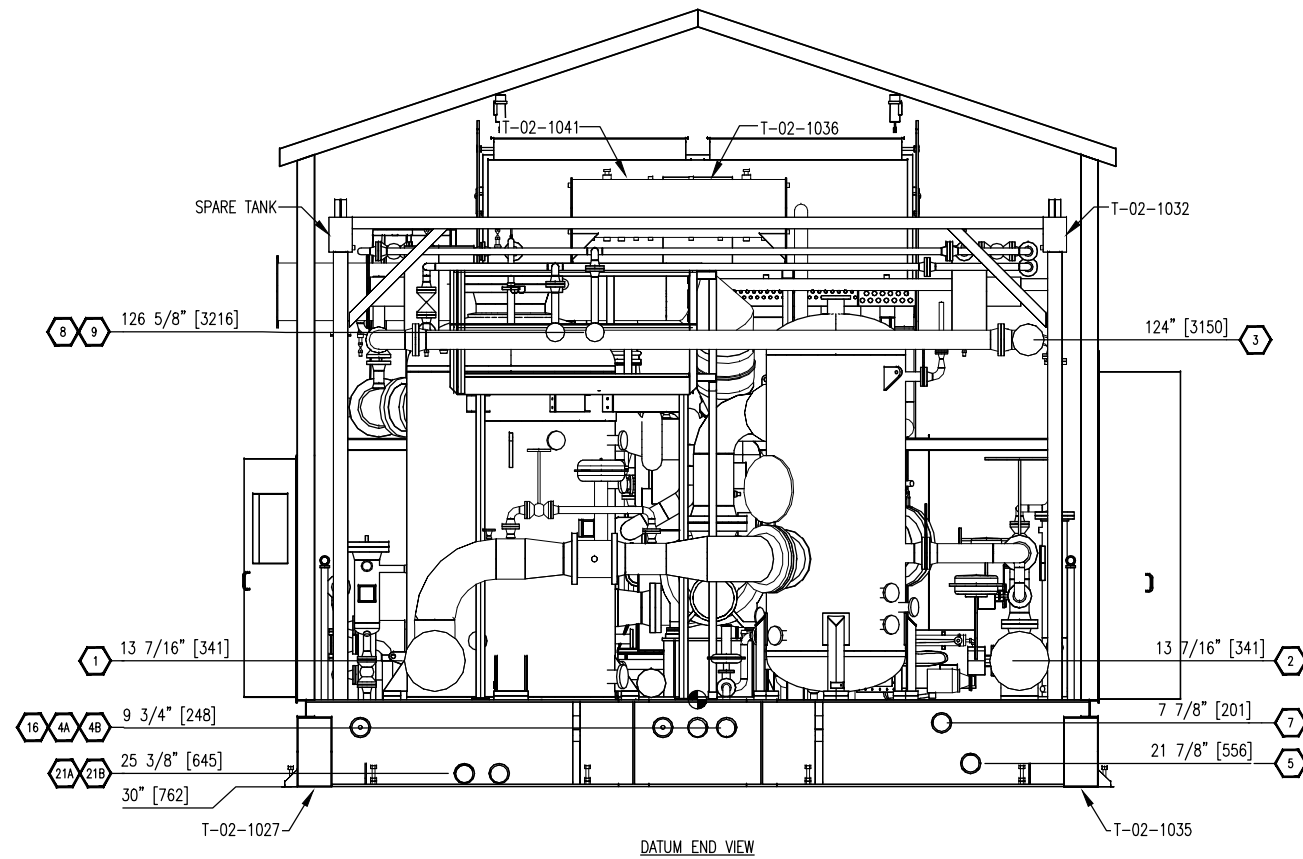
DATUM END VIEW
