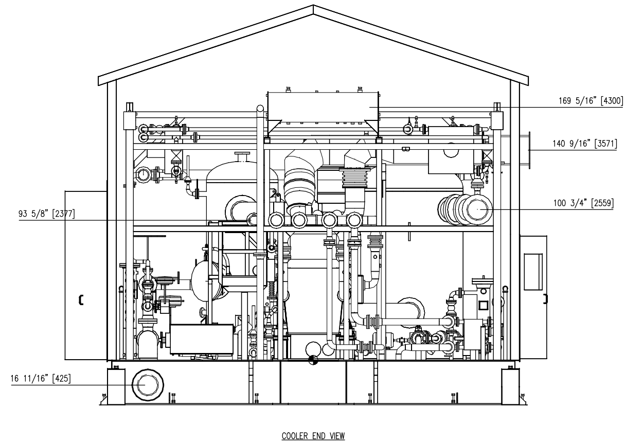
COOLER END VIEW
