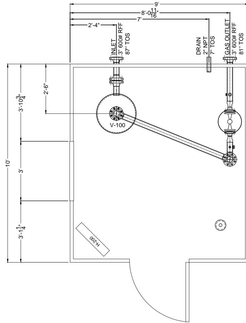
PLAN VIEW
