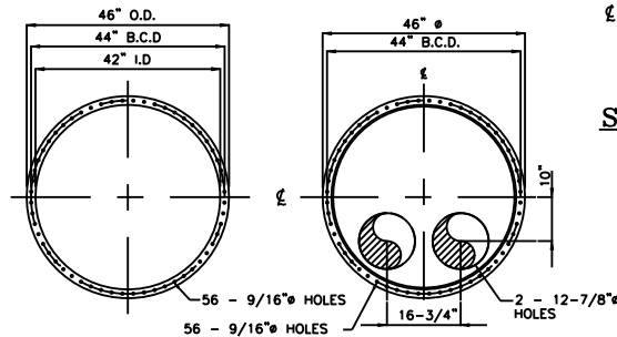
ITEM #8 DETAIL REQ'D 2
