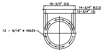
ITEM #11 DETAIL 3 - REQ'D
