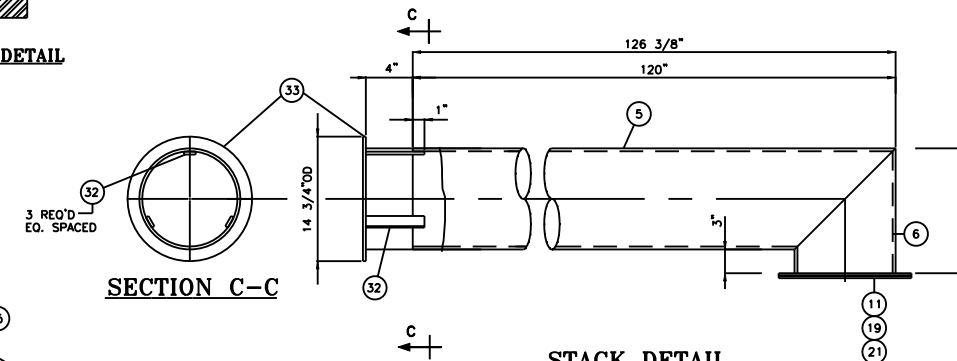
STACK DETAIL
