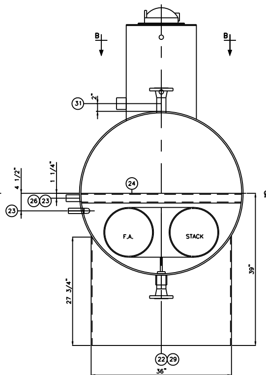
SECTION A - A HEATER SHELL & F.T. FLANGES NOT SHOWN
