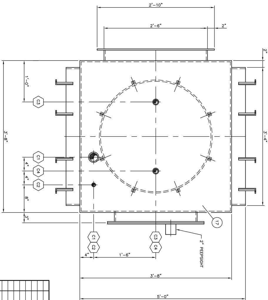
TOP VIEW OF ENARDO FLAMEBOX
