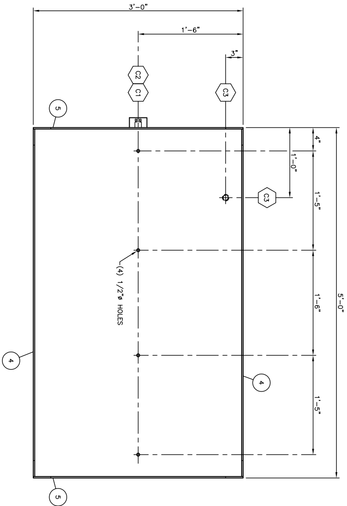
TOP VIEW
