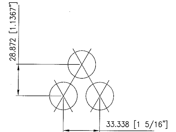
TUBE PATTERN
