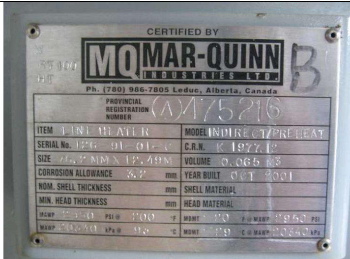
Data plate 1
