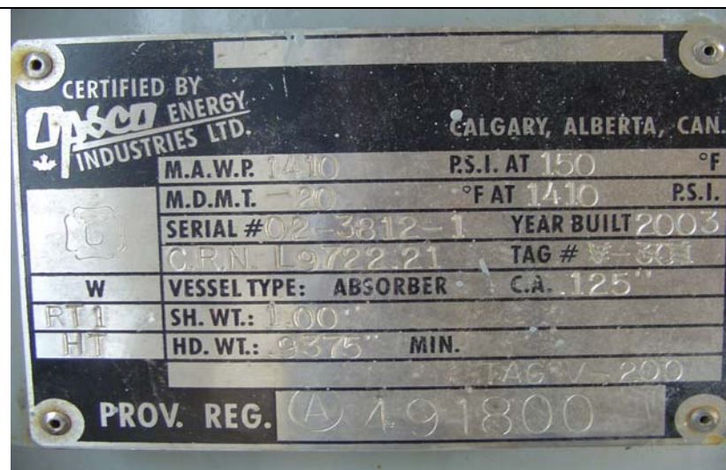
Data Plate
