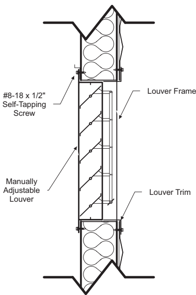
Louver Detail (TYP)
