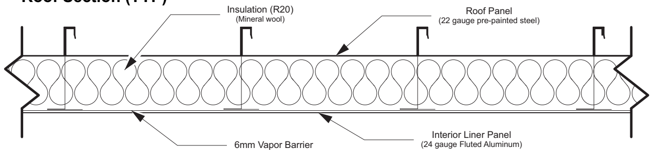
Roof Section (TYP)
