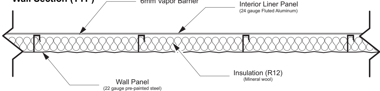
Wall Section (TYP)
