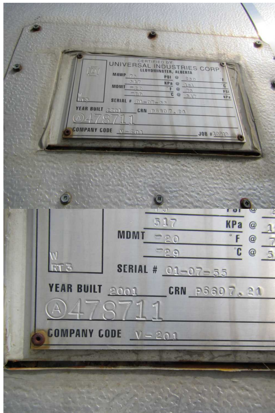
TREATER NAMEPLATE
