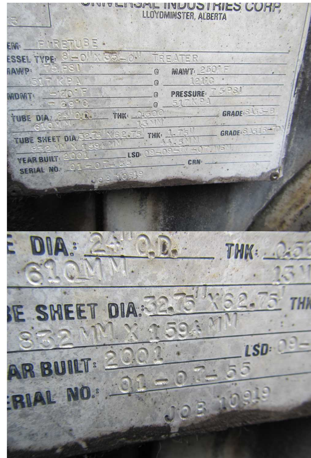
FIRETUBE NAMEPLATE
