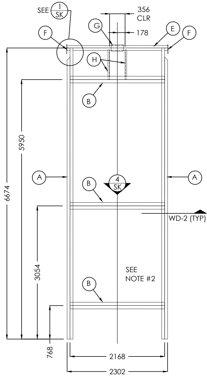
FRONT VIEW
