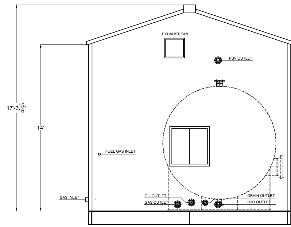
ORIENTATION VIEW B-B
