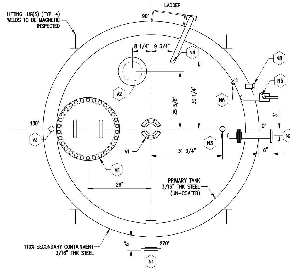
PLAN VIEW
